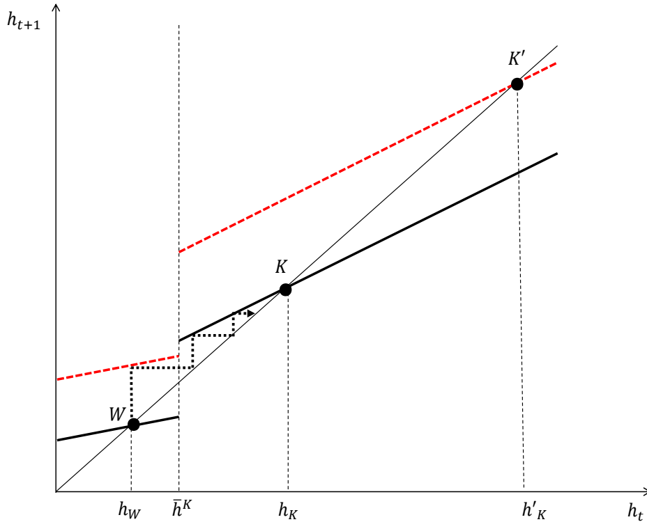
Figure 4: Transition to a Kafkaian equilibrium due to a temporary reduction in \ell
